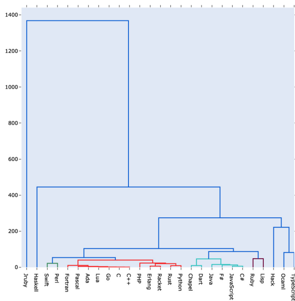
Fig. 5. Dendrogram representing Memory usage.
