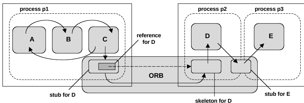
Figure 5.2. Performing non-local calls
