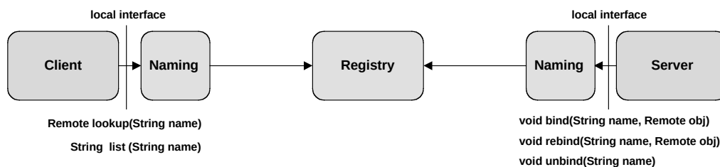
Figure 5.13. The RMI naming registry interface
