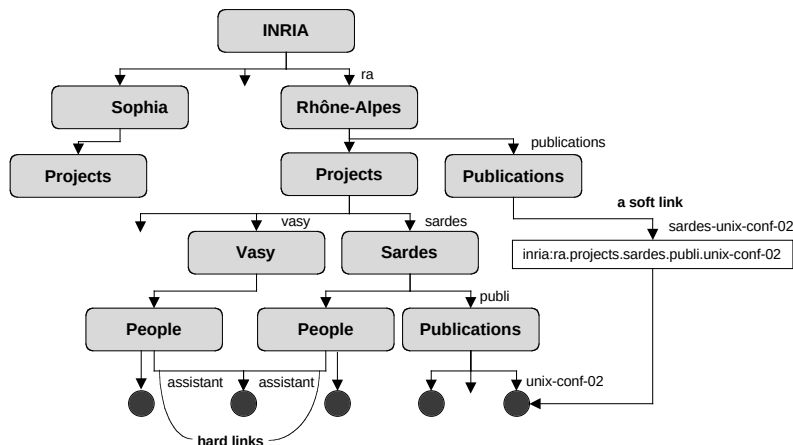
Figure 3.2. Hard and soft links
