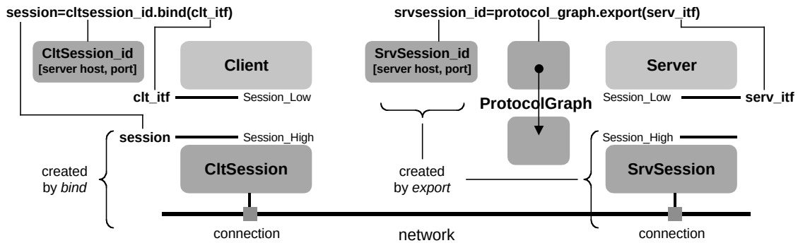
Figure 4.11. The export - bind pattern for session setup
