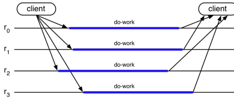
Figure 11.9. Active replication (adapted from [Guerraoui and Schiper 1997])
