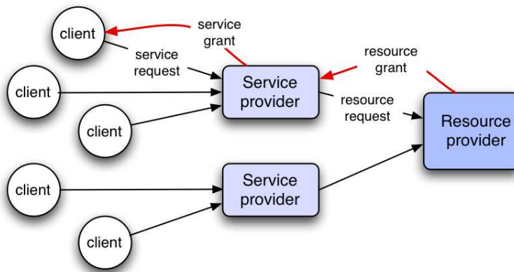
Figure 12.1. Service providers and resource providers
