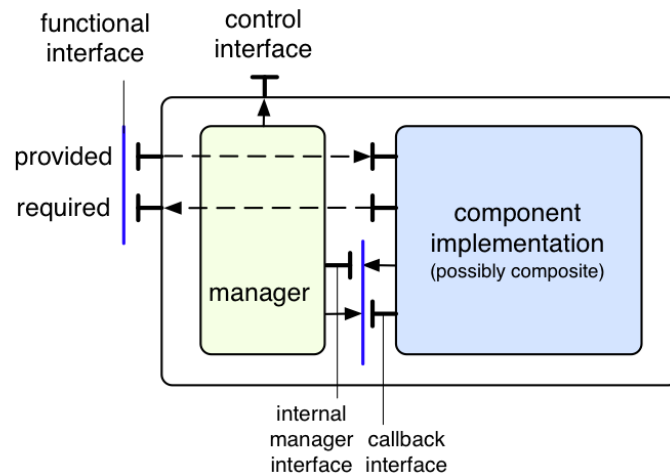
Figure 7.7. Component-manager interaction
