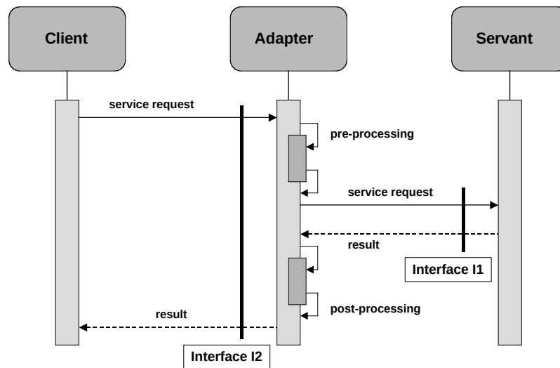
Figure 2.10. Adapter
