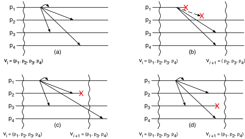
Figure 11.5. Virtual synchrony
