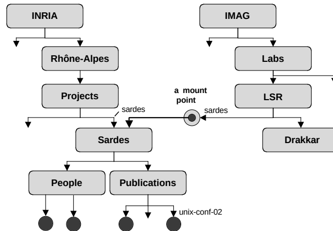
Figure 3.3. Mounting
