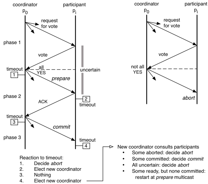
Figure 9.3. Three-phase commit
