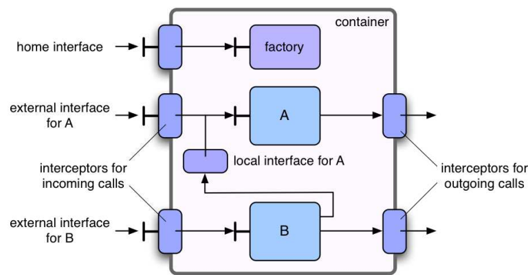
Figure 7.13. Container-mediated communication
