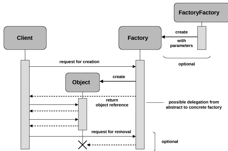
Figure 2.9. Factory
