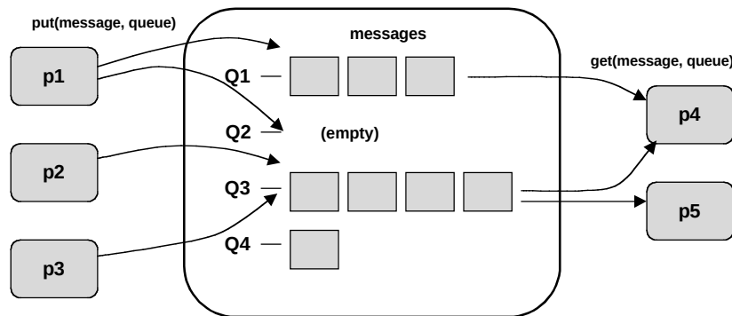
Figure 6.3. Message queuing
