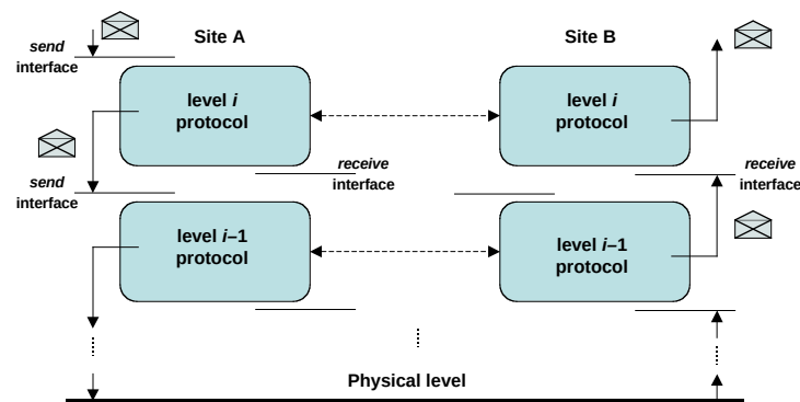
Figure 4.2. Protocol layering
