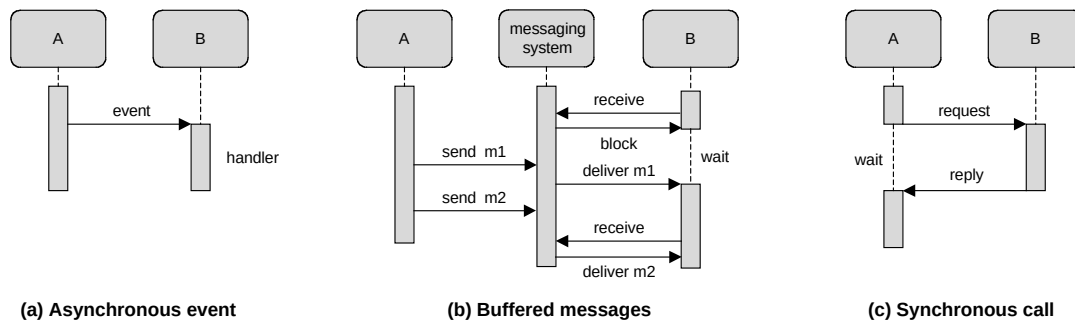
Figure 2.1. Some basic interaction mechanisms
