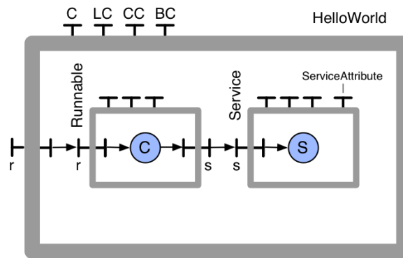
Figure 7.18. A simple Fractal application (from [Fractal ])
