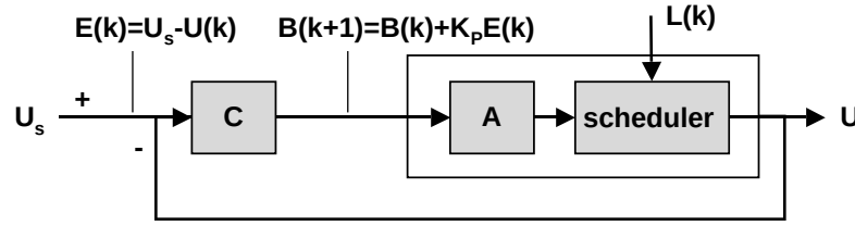
Figure 12.9. Feedback control of CPU scheduling
