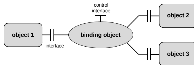
Figure 3.12. A binding object
