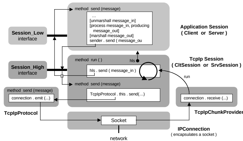
Figure 4.12. Sessions in the TCP-IP Jonathan framework
