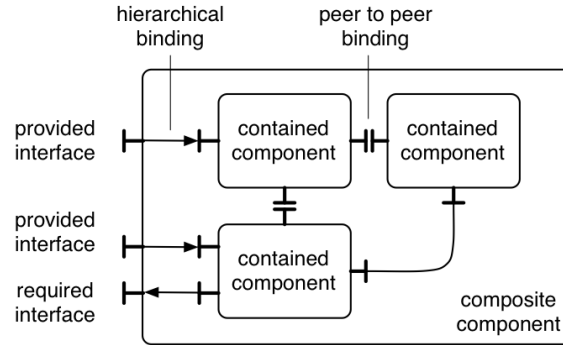
Figure 7.5. Bindings in a composite component
