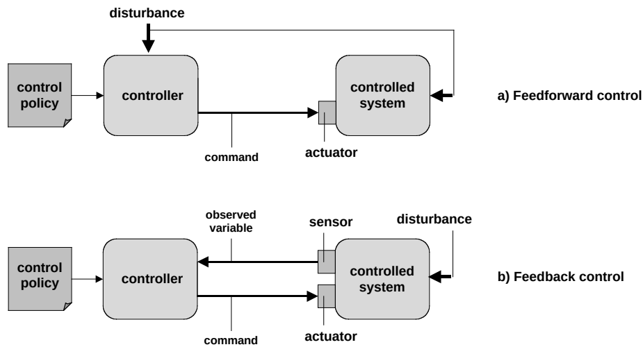
Figure 10.5. Two approaches to control
