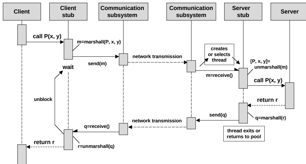
Figure 1.9. Remote procedure call: overall flow of control
