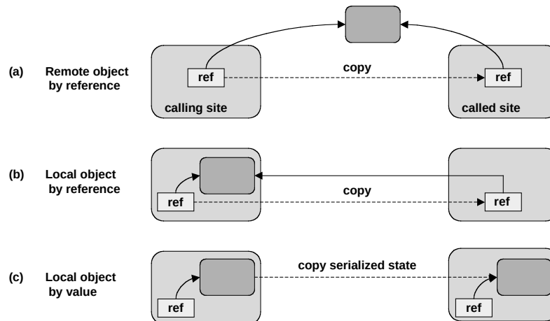
Figure 5.8. Passing an object as a parameter
