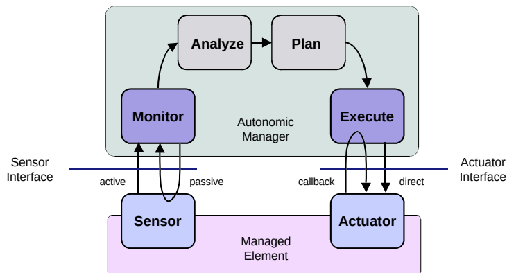
Figure 10.8. Interfaces for sensors and actuators
