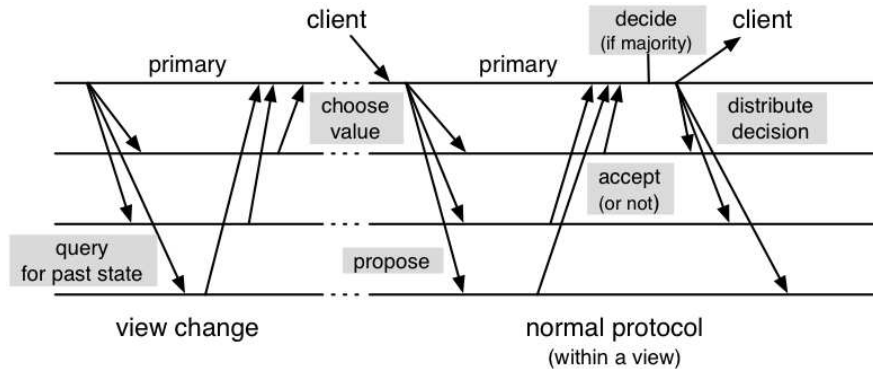
Figure 11.6. The Paxos consensus protocol
