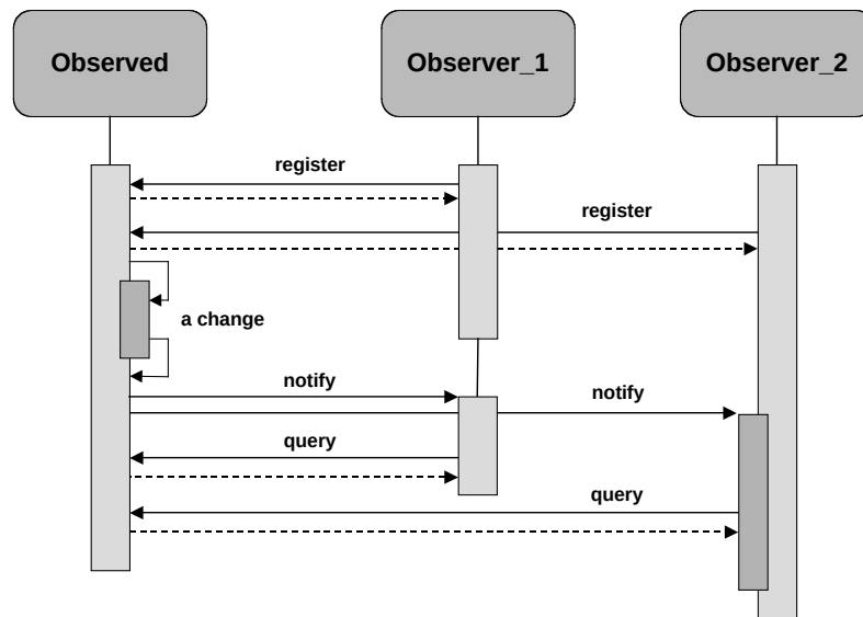
Figure 6.1. The OBSERVER pattern
