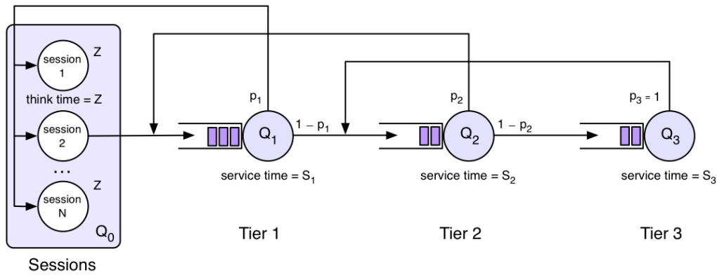
Figure 12.8. Queueing network for a 3-tier service (adapted from [Urgaonkar et al. 2007])
