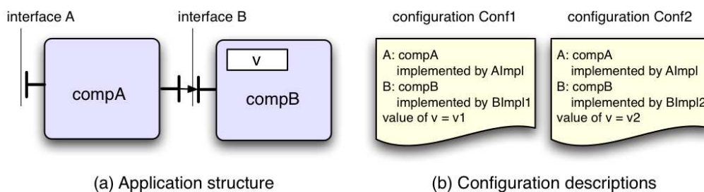
Figure 7.8. Organization of a simple application
