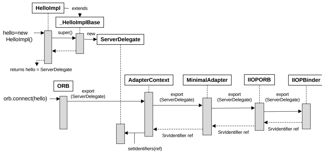
Figure 5.19. Exporting a servant in CORBA, phase 1
