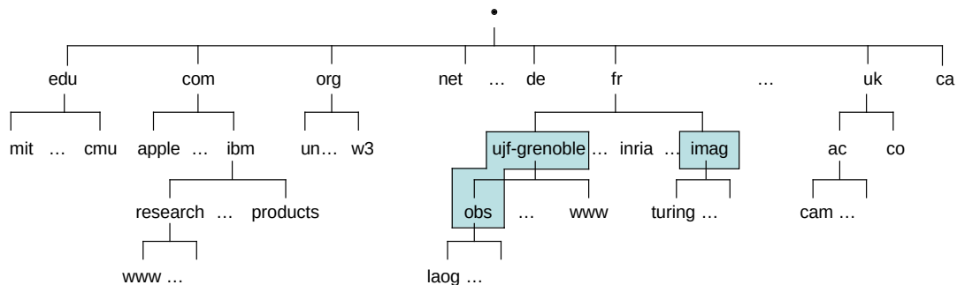
Figure 3.5. The DNS domain hierarchy
