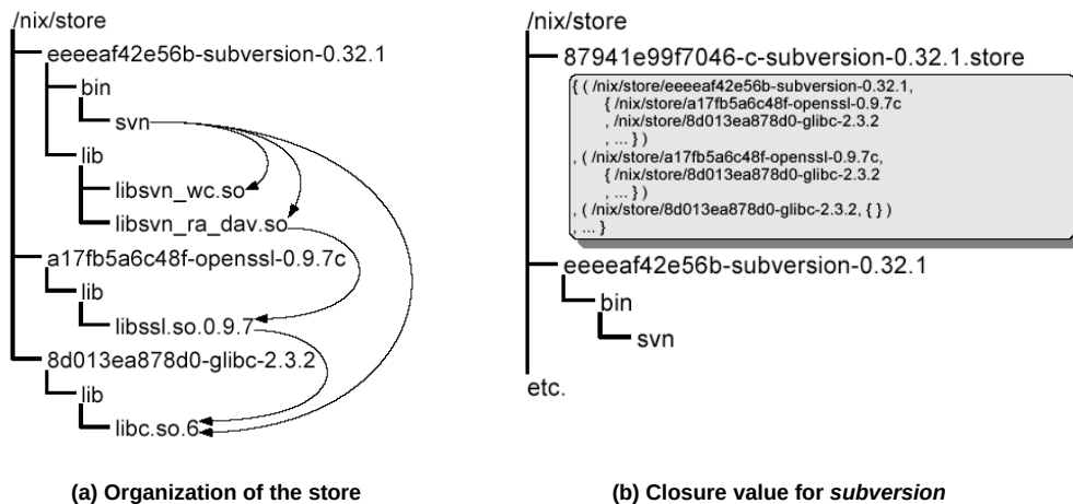
Figure 10.16. The Nix store, from [Dolstra et al. 2004b]
