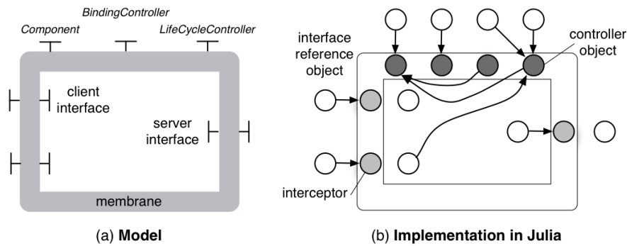
Figure 7.16. Controllers and interceptors in the Julia framework
