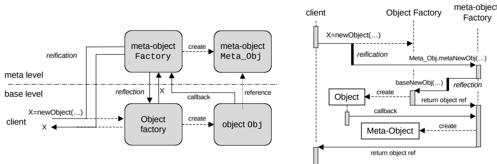
Figure 2.15. Object creation in a reflective system
