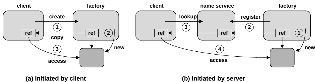
Figure 5.4. Object creation
