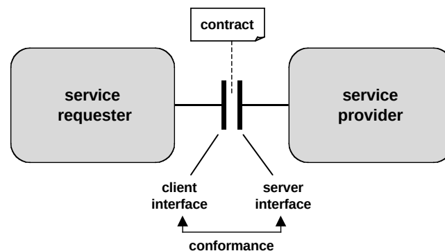
Figure 2.3. Interfaces
