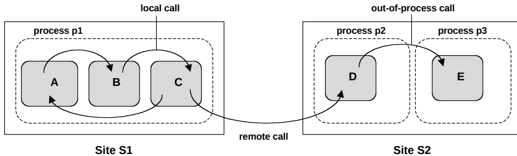
Figure 5.1. Distributed objects
