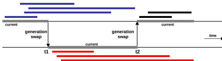
Figure 10.21. Quiescence detection
