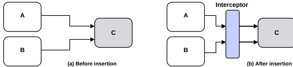
Figure 10.18. Dynamic interposition
