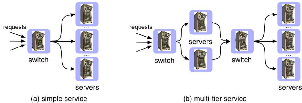
Figure 12.3. Load balancing
