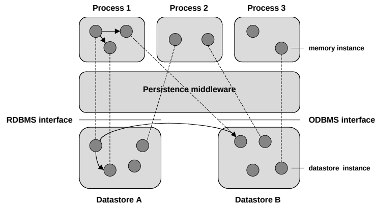
Figure 8.1. Persistence middleware
