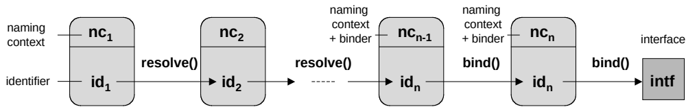
Figure 3.17. Resolving and binding identifiers in Jonathan
