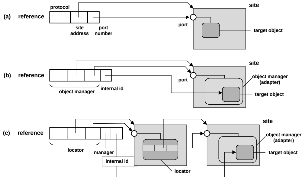
Figure 5.5. Object references
