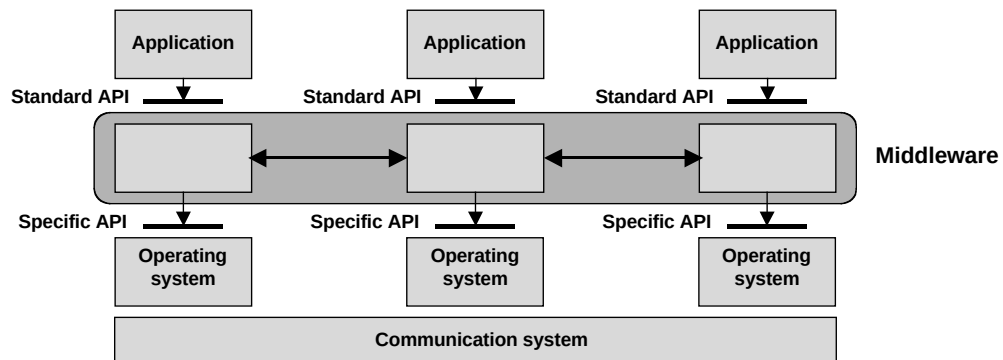
Figure 1.5. Middleware organization
