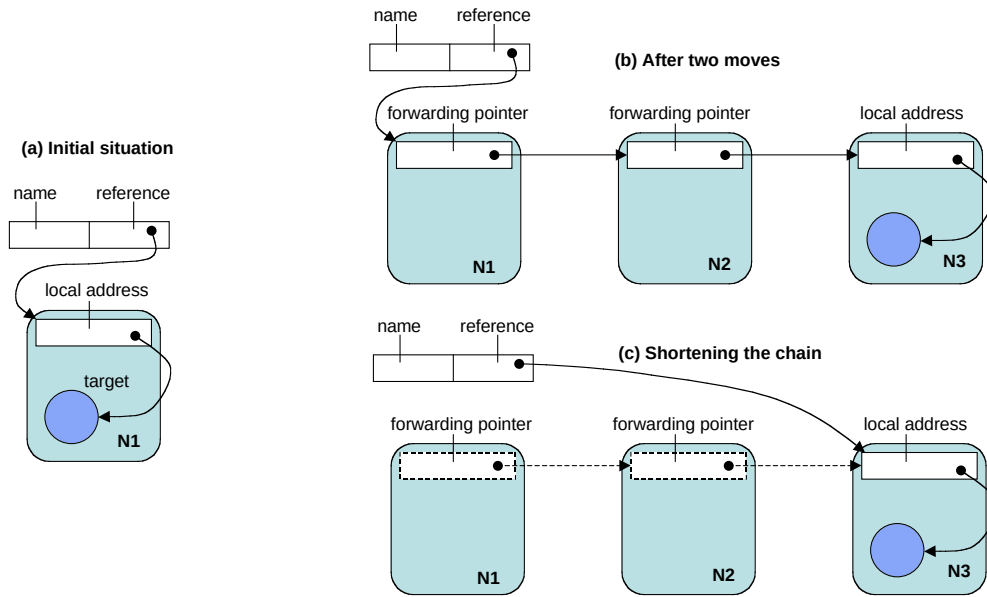
Figure 3.7. Forwarding pointers
