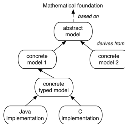
Figure 7.1. Component models
