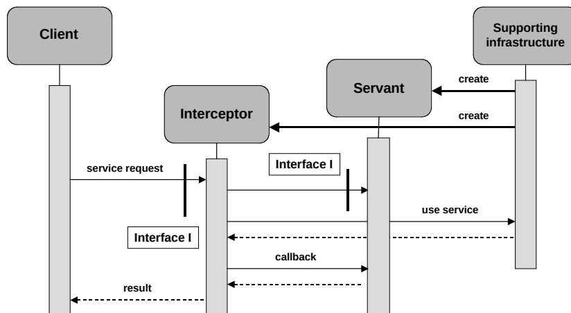
Figure 2.12. General Interceptor
