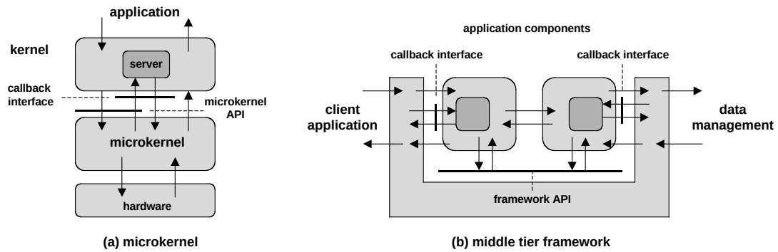
Figure 2.6. Framework architectures
