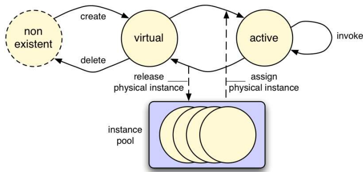
Figure 7.12. Instance pooling
