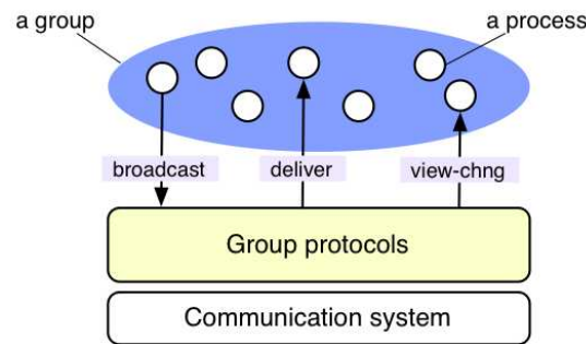
Figure 11.3. Group protocols
