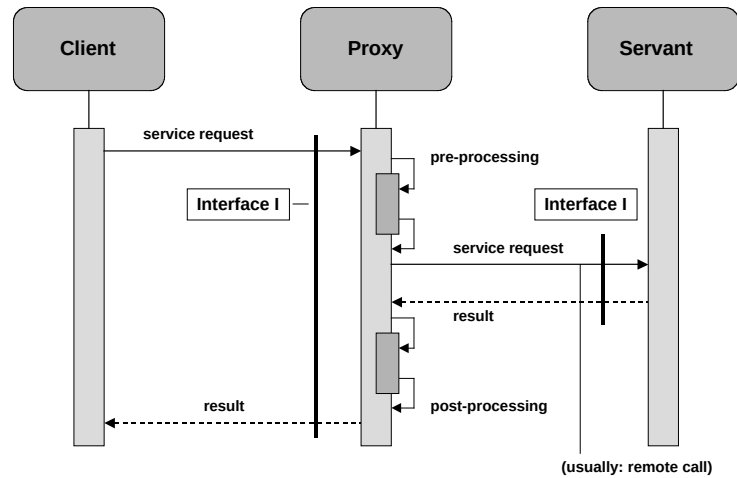
Figure 2.8. Proxy
