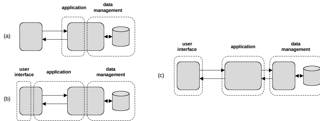
Figure 2.5. Multitier architectures
