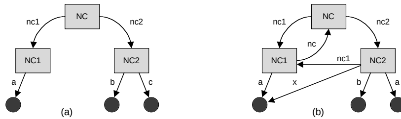
Figure 3.1. Naming contexts
