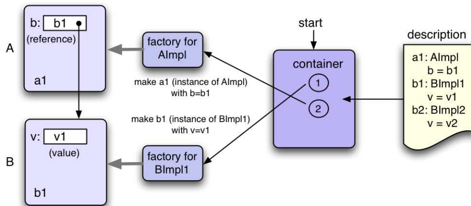
Figure 7.9. Inversion of control: constructor injection
