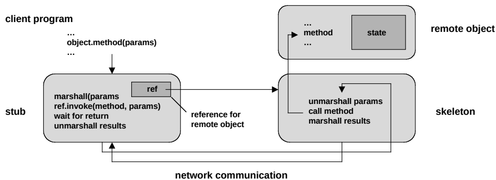
Figure 5.3. Invoking a remote object
