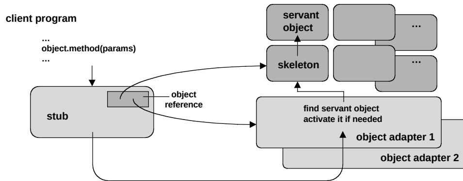
Figure 5.7. Invoking a remote object through an adapter
